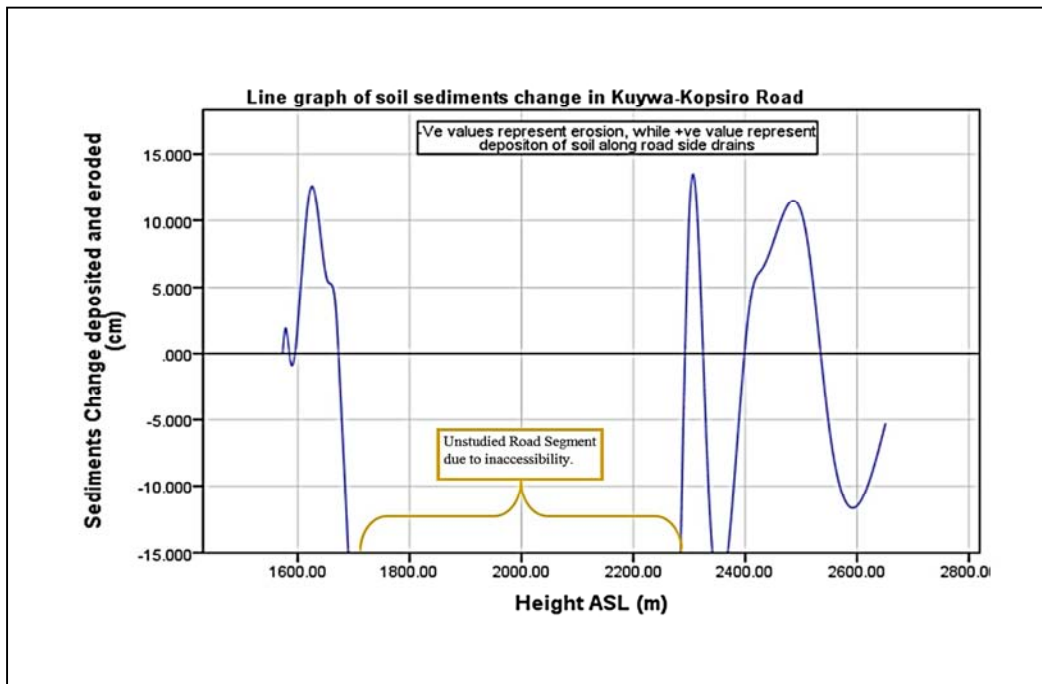
Figure 8. Sediments change deposited/eroded in Kuywa- Kopsiro road.
