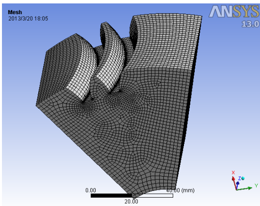
Figure 3. Boundary range division and grid division.
